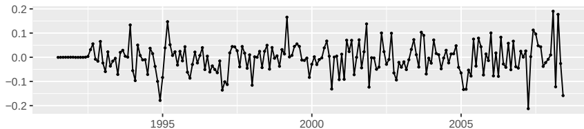
Residuals from ARIMA(2,1,3)(0,1,1)[12]
