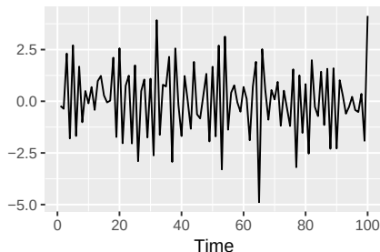
MA(2)
