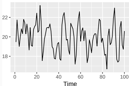
MA(1)
