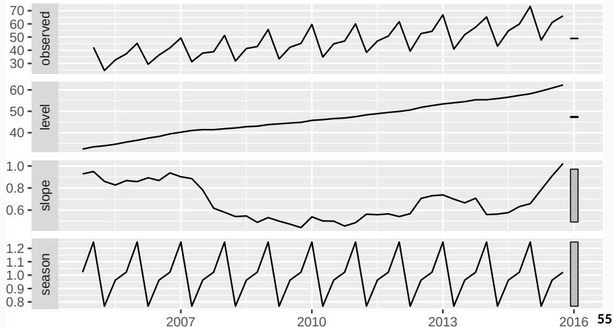
Components of ETS(M,A,M) method
