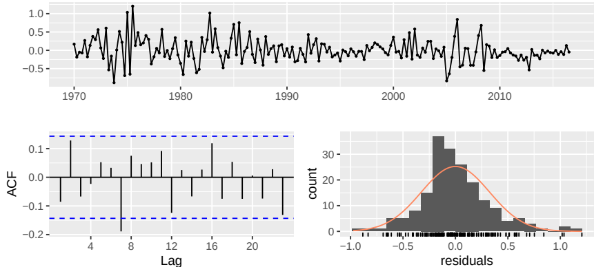
Residuals from Linear regression model
