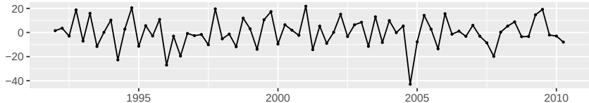
Residuals from Linear regression model
